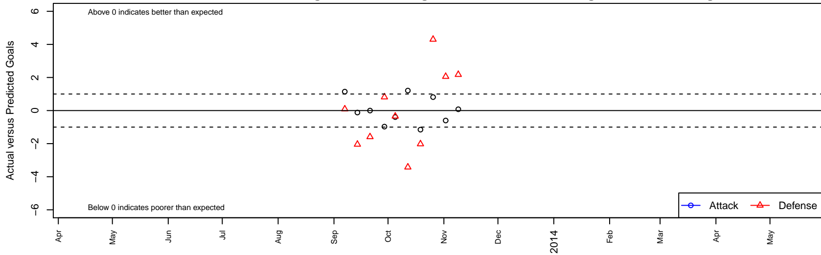
Storm FC Heuett–Nicol B02 Dots are actual minus expected GF (blue circles) and GA (red triangles). Blue line is smoothed change in attack strength. Red is smoothed change in defense strength.
